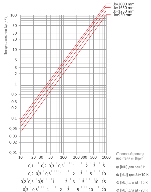
VKN1-6,5/17/Lk VKN1-9/17/Lk
